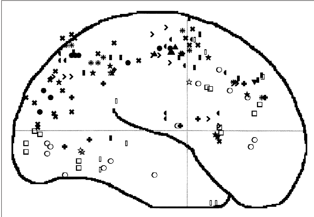
Fig. 2. Schematic of the right side of the cortex, showing regions of activation for spatial (filled symbols) and object (open symbols) working memory tasks in humans (adapted from Smith & Jonides, 1999). The results are drawn from 11 different experiments, with different symbols being used for different experiments. Not all the activations occurred on the surface of the brain, so the schematic should be interpreted as a glass brain—as though one were looking through the brain from the side.
